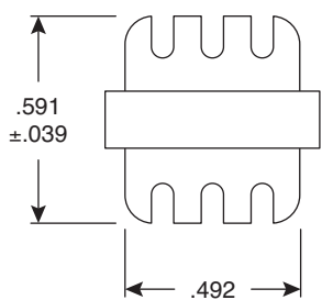
Dimensions (In.)
